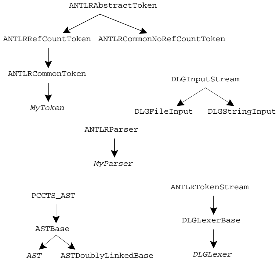
FIGURE 3 C++ Class Hierarchies
